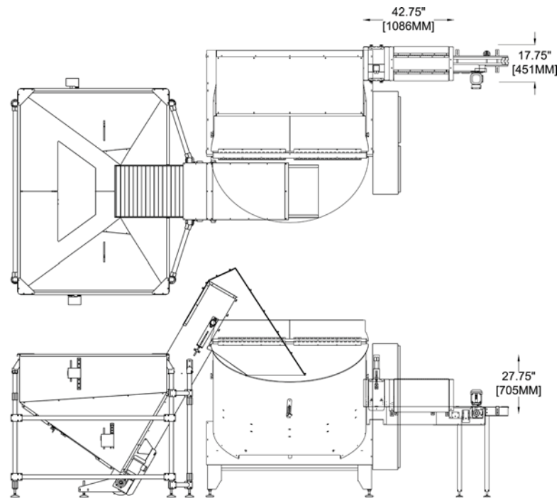
NECO-ORIENTER 180 Integrated with Bottle Unscrambler
